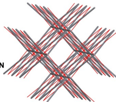
inclined catenation of sq1 (red) + 6-c extended ring net (grey) ERN
