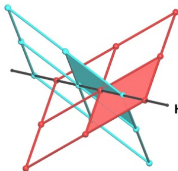
inclined catenation of two sq1 + Hopf ring net (HRN) 2-c linear chain
