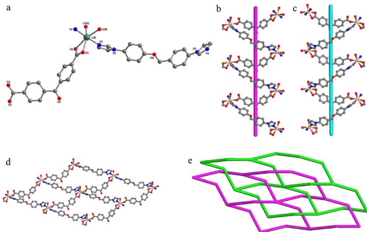
[\text{Cd}(\text{cba})(\text{ibpi})] (101 пример)
