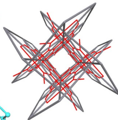
inclined catenation of hcb (red) + 8-c extended ring net (grey) ERN
