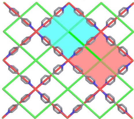
underlying net (red) sq1 + fused ring net (green) FRN sq1
