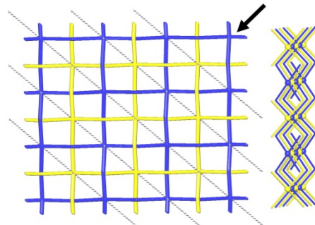
101 structures ERN (4,4)IIb
